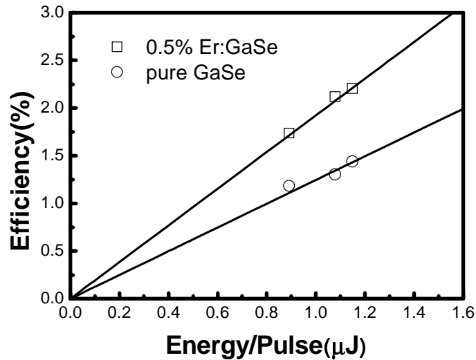
Fig. 6. Comparison of the SHG conversion efficiencies of pure and 0.5% Er:GaSe crystals with identical crystal length.
