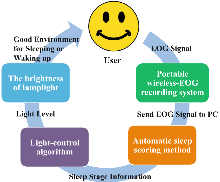
Fig. 1. The concept and architecture of the proposed adaptive light system.
