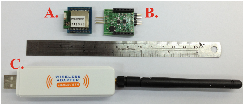
Fig. 2. The three components of the portable wireless-EOG recording unit.
