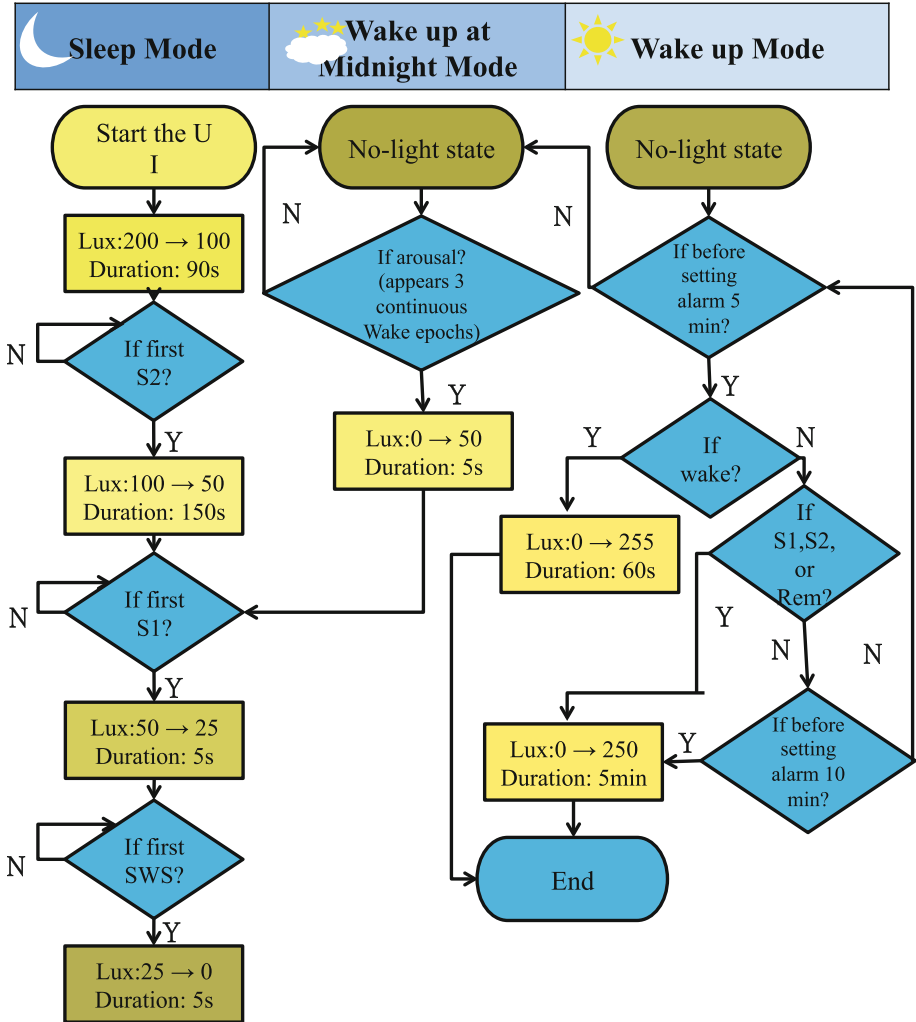
Fig. 3. The flowchart of our light control algorithm, which has three modes: sleep, wake up at the middle of the night, and wake up.
