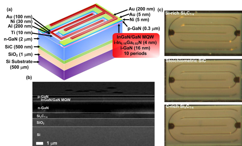
Figure 7. The structure of the GaN LED on SiC/SiO 2 /Si substrates. (a) The structure diagram of the GaN LED on SiC/SiO 2 /Si substrates (b) The SEM image of the GaN LED devices grown on the SiC/SiO 2 /Si substrate. (c) The photograph of the GaN LED devices grown on the SiC/SiO 2 /Si substrate with Si-rich (Upper), the stoichiometric (Middle), and C-rich (Lower) Si x C 1-x films.
