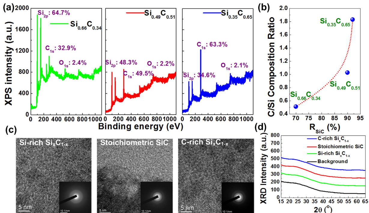
Figure 2. Material characteristic of \text{Si}_x\text{C}_{1-x} film. (a) The XPS spectra of the Si-rich, the stoichiometric, and C-rich \text{Si}_x\text{C}_{1-x} films. (b) The C/Si composition ratio of the \text{Si}_x\text{C}_{1-x} film as a function of R_{\text{SiC}} . (c) FETEM image, SAD pattern and (d) XRD spectra of the Si-rich, the stoichiometric, and C-rich \text{Si}_x\text{C}_{1-x} films.
