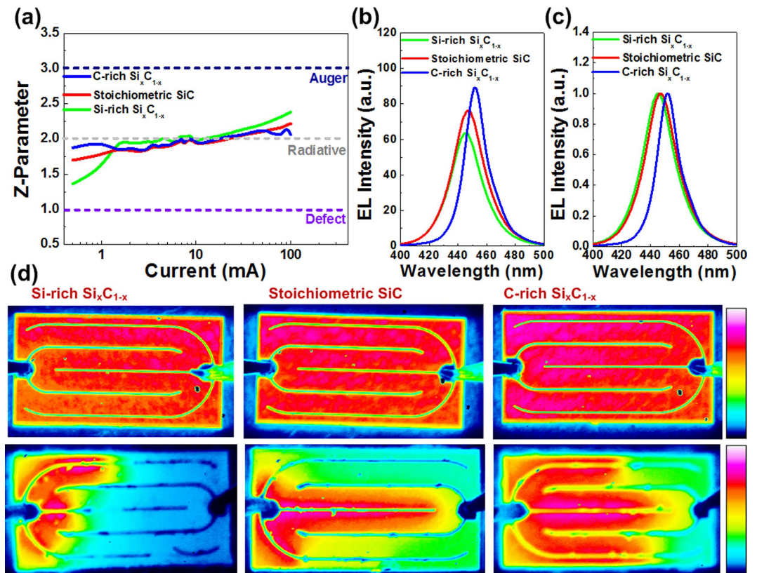
Figure 4. The EL characteristic of GaN LEDs grown with different C/Si composition ratio based \text{Si}_x\text{C}_{1-x} films. (a) The Z-parameter, (b) the EL spectra and (c) normalized EL for the GaN LEDs grown with different C/Si composition ratio based \text{Si}_x\text{C}_{1-x} films. (d) The EL intensity distribution of the GaN LEDs grown with different C/Si composition ratio based \text{Si}_x\text{C}_{1-x} films under the operating current of 1 mA (Upper) and 100 mA (Lower).
