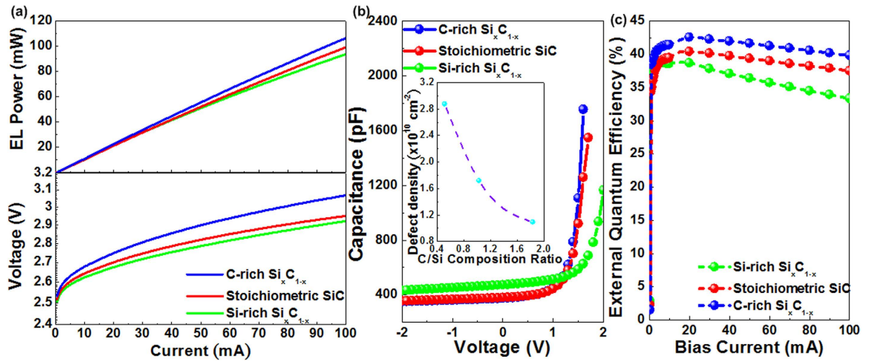
Figure 3. The electrical characteristics of GaN LEDs grown with different C/Si composition ratio based Si x C 1-x films. (a) The V-I (Lower) and P-I (Upper) characteristics, (b) C-V characteristics, defect density (Inset), and (c) EQE of the GaN LEDs grown with different C/Si composition ratio based Si x C 1-x films.
