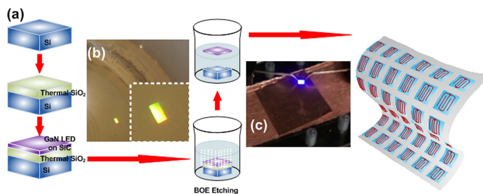
Figure 8. Lift-off process for the GaN LED grown upon a-Si x C 1-x /SiO 2 /Si substrate. (a) Fabrication procedure for lifting off the GaN LED. Inset: the two photographs show that (b) the GaN LED on a-SiC buffer being lifted off under a buffer oxide etching (BOE) solution, and (c) the exfoliated GaN LED on a-SiC buffer transferred on copper substrate.
