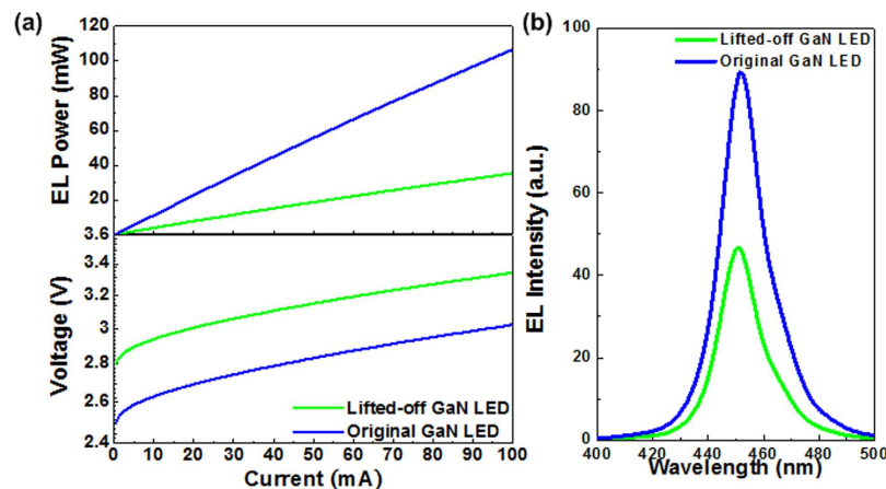
Figure 6. The EL characteristic of the lifted-off GaN LEDs. (a) The V-I (lower) and P-I (upper) responses and (b) The EL spectrum of the lifted-off GaN LED on a-Si x C 1-x buffer transferred onto the copper substrate and the original GaN LED on a-Si x C 1-x buffer.
