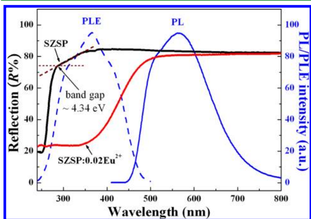
Figure 5. Diffuse reflectance spectra of \text{Sr}_8\text{ZnSc}(\text{PO}_4)_7 (black line) and \text{Sr}_8\text{ZnSc}(\text{PO}_4)_7:\text{0.02Eu}^{2+} (red line), and PL/PLE spectra of \text{Sr}_8\text{ZnSc}(\text{PO}_4)_7:\text{0.02Eu}^{2+} phosphor.
