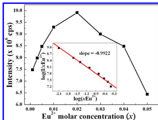
Figure 4. Concentration dependence of emission intensity of \text{Sr}_8\text{ZnSc}(\text{PO}_4)_7:x\text{Eu}^{2+} ( x = 0.001\text{--}0.05 mol) under 400 nm excitation. The inset illustrates the I/x dependence on x on a logarithmic scale.
