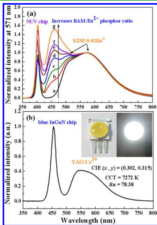
Figure 7. EL spectrum of white LEDs composed of (a) 400 nm NUV chip and a phosphor blend of \text{BaMgAl}_{10}\text{O}_{17}:\text{Eu}^{2+} and \text{Sr}_8\text{ZnSc}(\text{PO}_4)_7:0.02\text{Eu}^{2+} in various mixing ratios; (b) InGaN chip pumped with \text{YAG}:\text{Ce}^{3+} phosphor, driven by 350 mA current.
