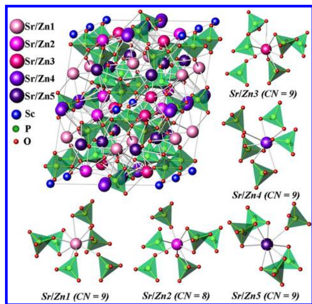
Figure 2. Crystal structure of \text{Sr}_8\text{ZnSc}(\text{PO}_4)_7 .
