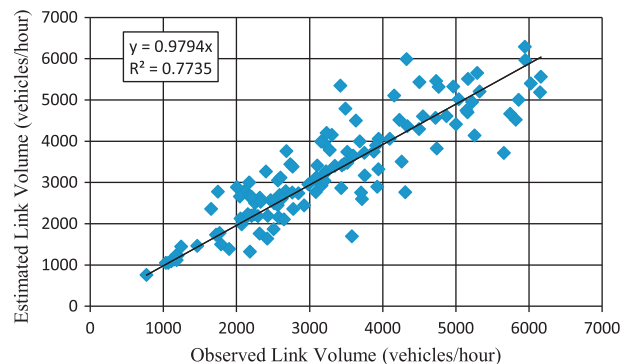
Fig. 20. Observed vs. estimated link volume on freeway links on the triangle regional model, NC network.
