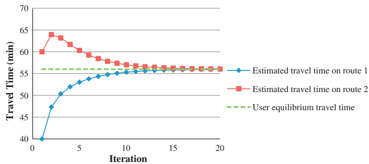
Fig. 10. Path travel time convergence pattern as a function of inner iteration number.
