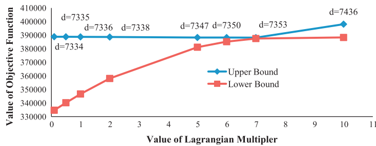
Fig. 12. Upper bound and lower bound of objective function as a function of Lagrangian multiplier.
