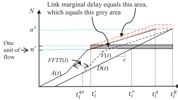
Fig. 5. Illustration of link marginal delay on a congested link.
