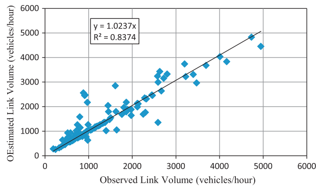
Fig. 21. Observed vs. estimated link volume on highway and arterial links on the triangle regional model, NC network.
