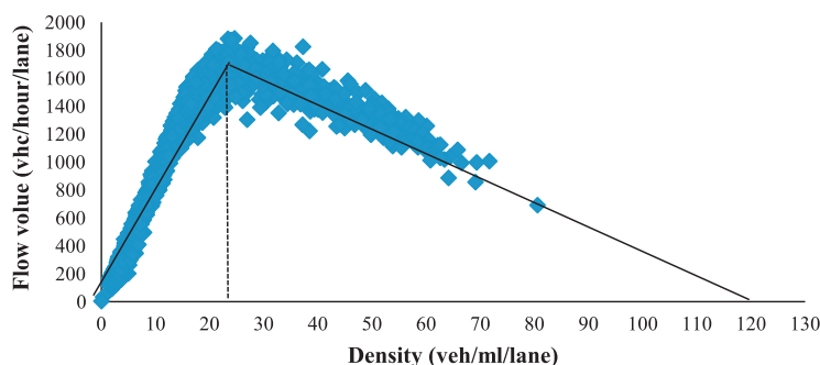
Fig. 14. Triangular relationship between flow and density at sensor b .
