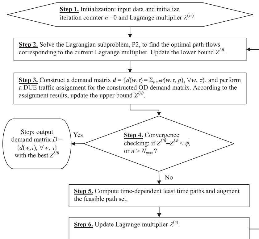
Fig. 4. Flowchart of the Lagrangian Relaxation-based heuristic.
