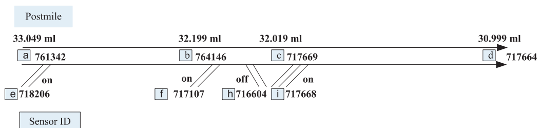
Fig. 13. Network representation of a section of I-210 West bound corridor.
