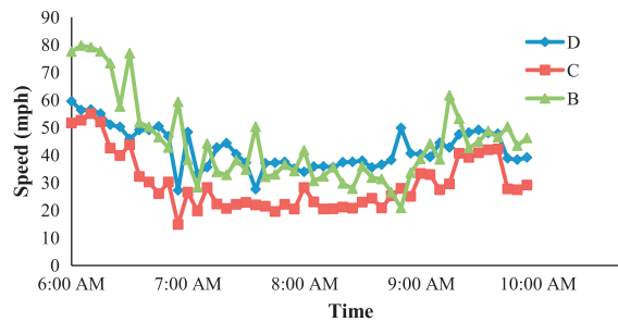
Fig. 15. Observed speed time series on freeway stations (demonstrating a congested period from 7:00 AM to 9:00 AM).
