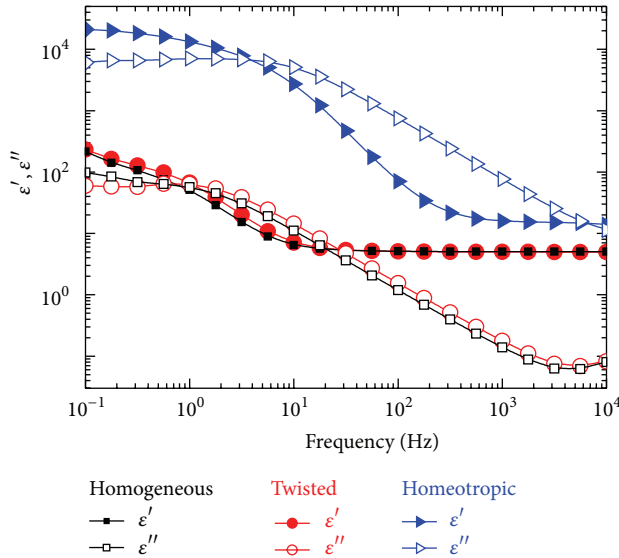
FIGURE 6: The dielectric spectra of E7 in homogeneous, twisted, and homeotropic cells at 296 K.
