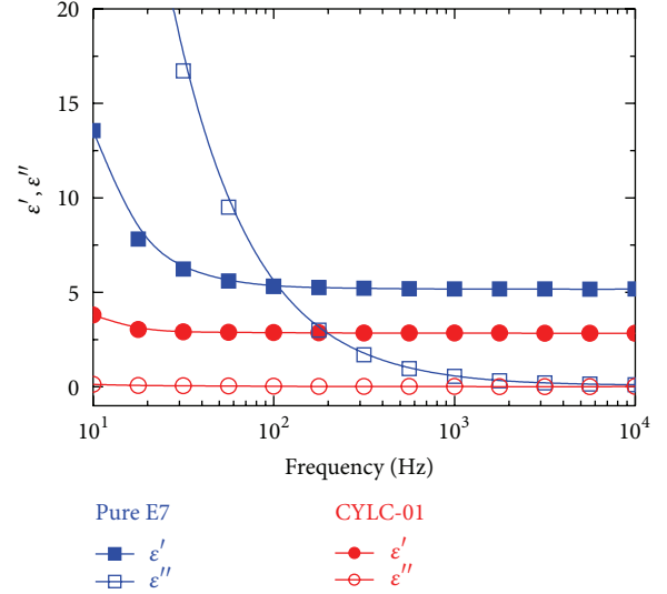
FIGURE 1: The dielectric spectra of the low-resistivity NLC E7 and high-resistivity NLC CYLC-01 confined in homogeneous cells at 303 K. \epsilon' and \epsilon'' are the real and imaginary parts of the complex dielectric function.
