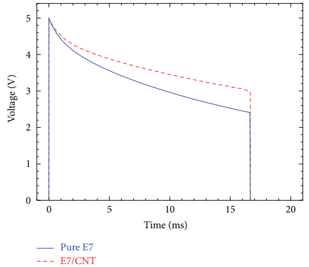
FIGURE 4: Voltage responses of doped and undoped E7 cells to a 5-V square-wave pulse of 15.6 \mu\text{s} .
