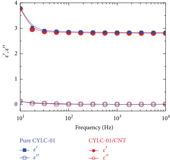
FIGURE 2: The dielectric spectra of pristine and 0.05 wt% CNT-doped CYLC-01 in homogeneously aligned cells at 303 K.
