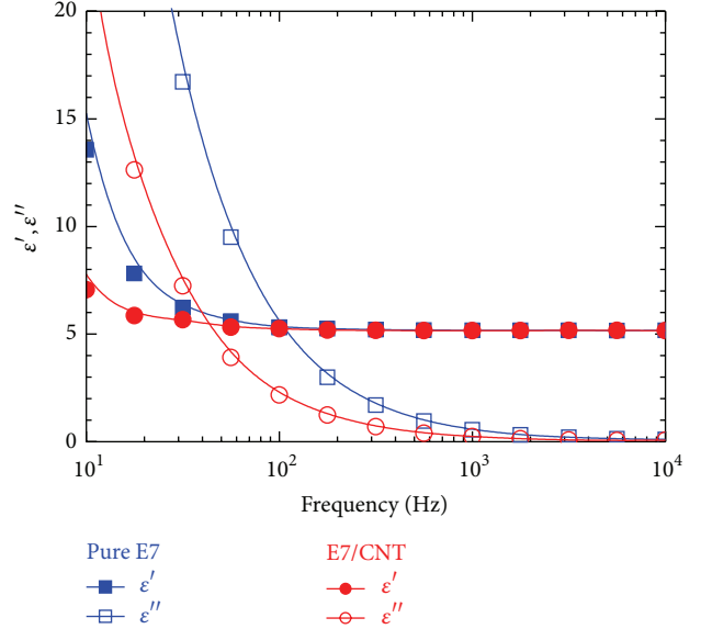
FIGURE 3: The dielectric spectra of pure and 0.05 wt% CNT-doped E7 in homogeneous cells at 303 K.
