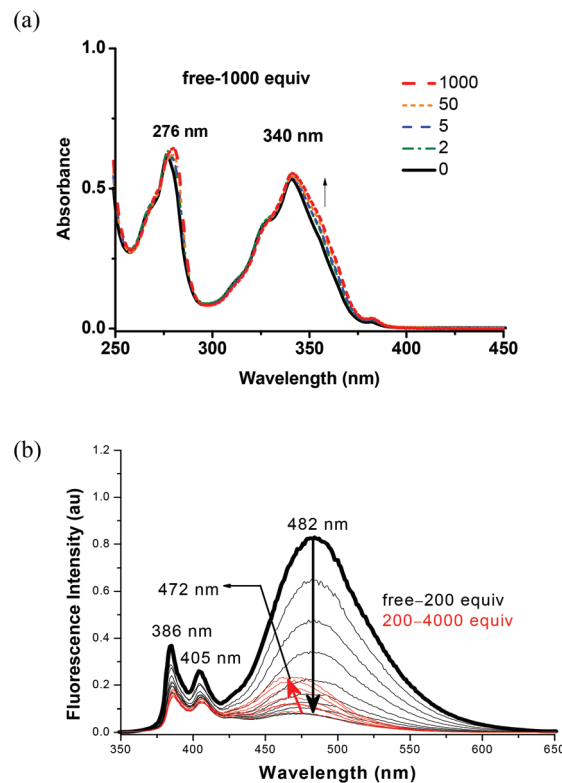
Fig. 2 Changes in the (a) UV-vis and (b) fluorescent emission spectra ( \lambda_{\text{ex}} = 326 \text{ nm} ) of 4 ( 10 \mu\text{M} ) upon addition of various concentrations of \text{AcO}^- in \text{CH}_3\text{CN} at 25 \text{ }^\circ\text{C} .
