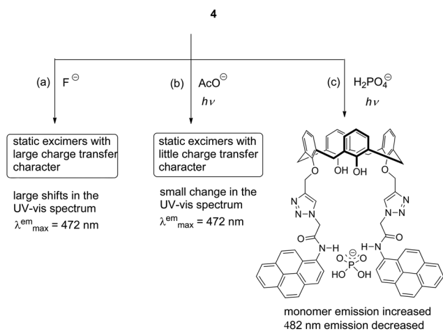
Scheme 2 Three binding modes of 4 with anions in \text{CH}_3\text{CN} .
