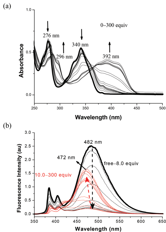
Fig. 1 Variation of the (a) UV-vis absorption and (b) fluorescent emission spectra ( \lambda_{\text{ex}} = 326 \text{ nm} ) of 4 ( 10 \mu\text{M} ) upon addition of various concentrations of \text{F}^- in \text{CH}_3\text{CN} at 25 \text{ }^\circ\text{C} .
