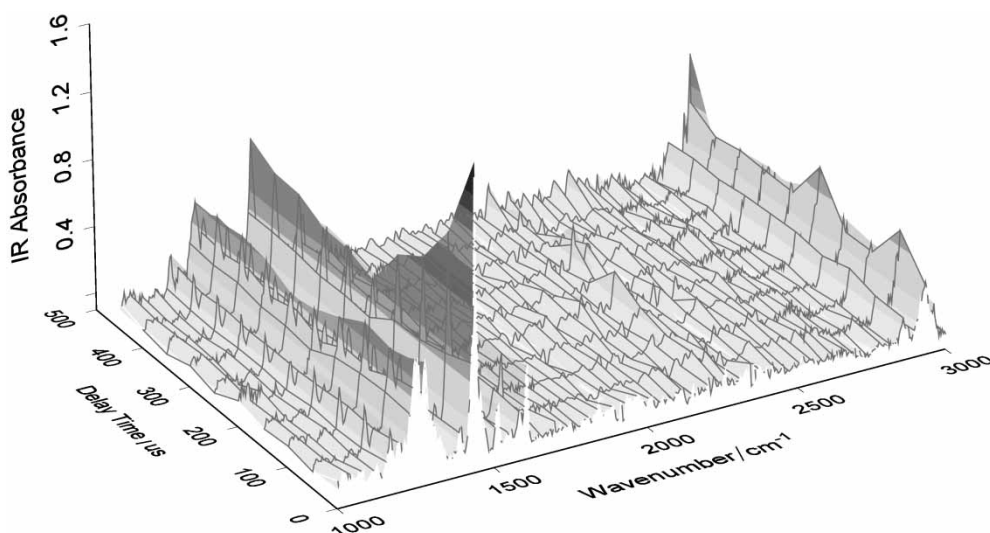
Figure 10. Time-resolved FTIR spectra taken from an SSFLC excited by a +10V pulse extending from 0 to 110 μs.
