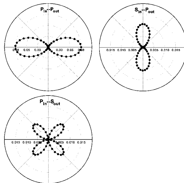
Figure 3. Theoretical curves of azimuthal patterns of second harmonic generation for an SSFLC cell with various optical beam polarization combinations.
