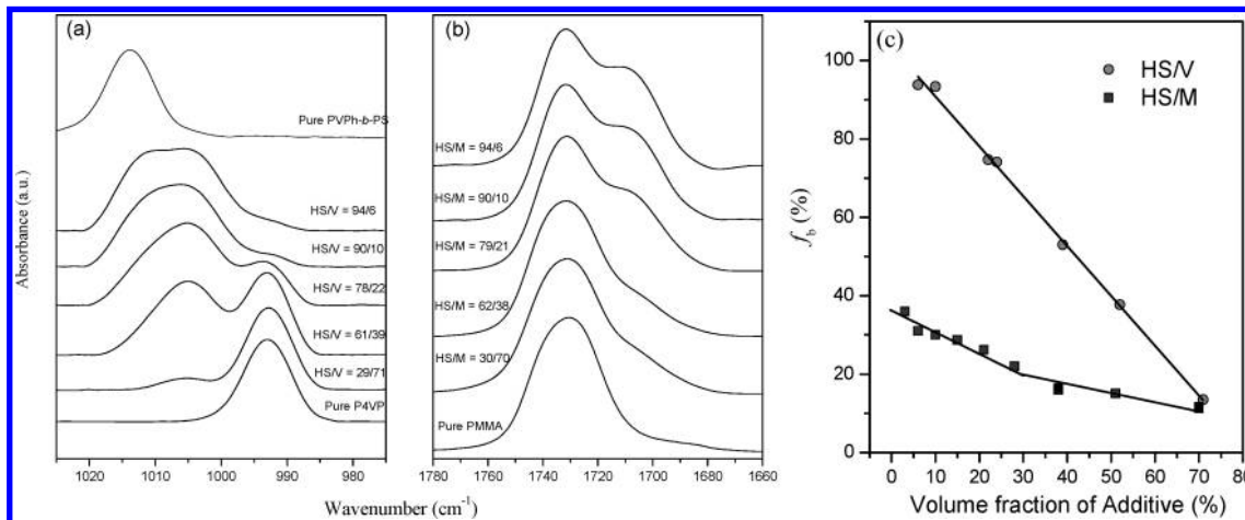
Figure 1. FTIR spectra recorded at 120 °C in (a) the pyridine absorption region for the HS/V blends and (b) the C=O absorption region for the HS/M blends. The compositions are indicated above the respective profiles. (c) The corresponding f_b values for the fraction of hydrogen-bonded groups. Lines drawn over the data points are only for eye-guiding. The decrease in f_b , (i.e., reduction of hydrogen bonding efficiency) with the increase in the homopolymer volume fraction reveals a systematically decreased miscibility in both blends.
