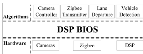
Fig. 5. The system architecture of LVWS.
