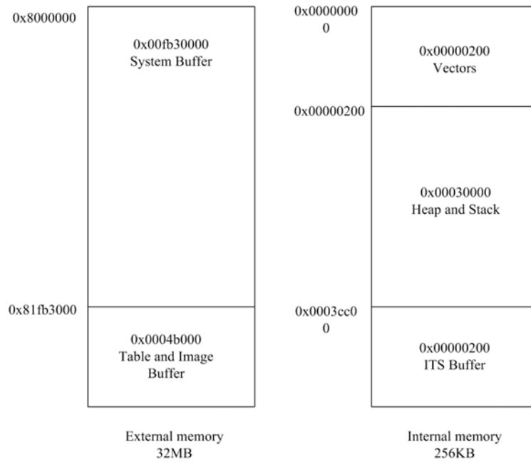
Fig. 14. Memory allocation.
