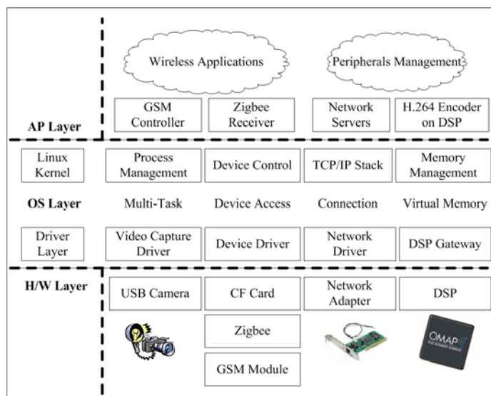
Fig. 6. The system architecture of MSR.
